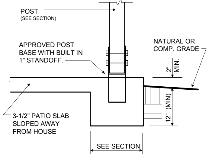
TYPICAL FOOTING DETAIL - "D"
