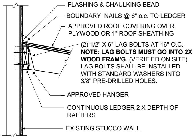
LEDGER CONNECTION - "A"
