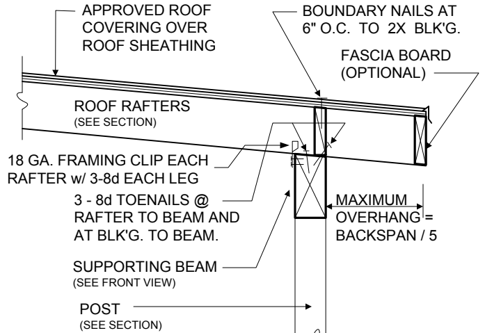
RAFTER TO BEAM DETAIL - "B"
